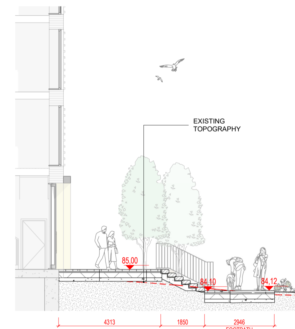
6 Section 06 1: 100 @A1
