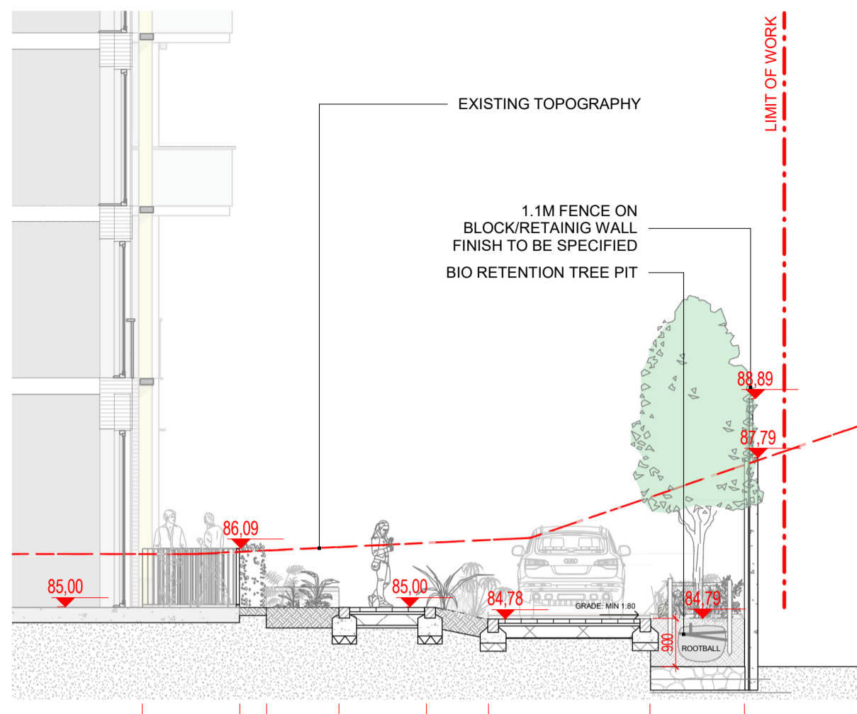
1 Section 01 1: 100 @A1
