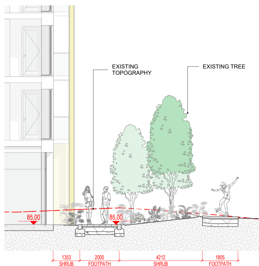
4 Section 04 1: 100 @A1
