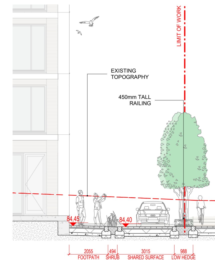
8 Section 08 1: 100 @A1
