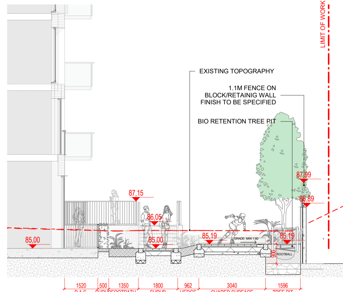
2 Section 02 1: 100 @A1
