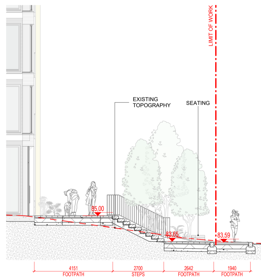
5 Section 05 1: 100 @A1
