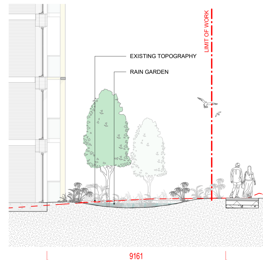
3 Section 03 1: 100 @A1
